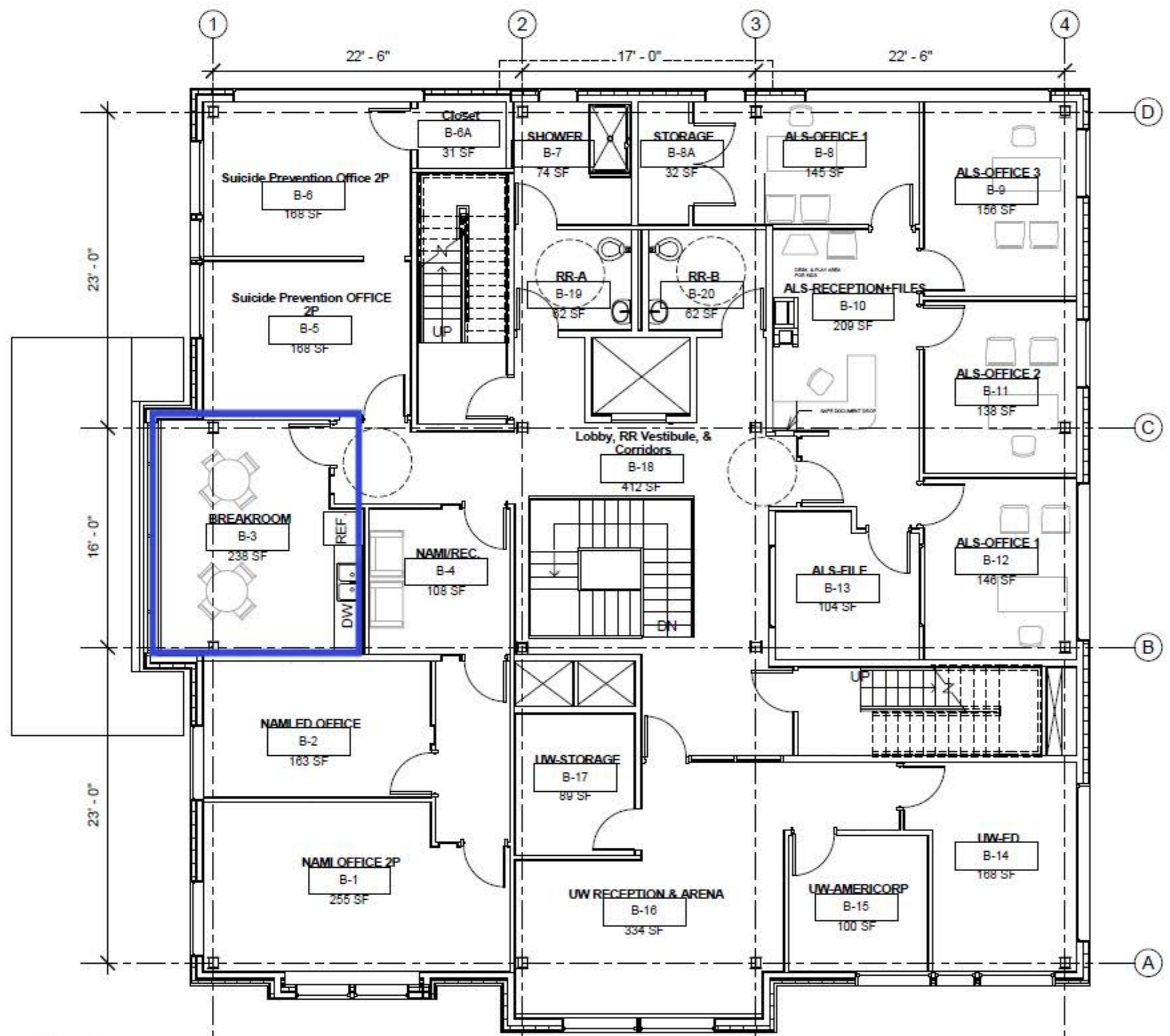
1 Level 2 1/8" = 1'-0"
